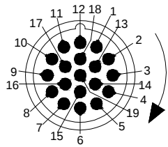
MALE END VIEW
